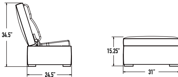
Custom and Standard Jumpseat Specifications.
