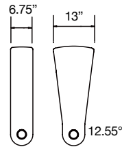
Straight and Wedge Arm Connectors
