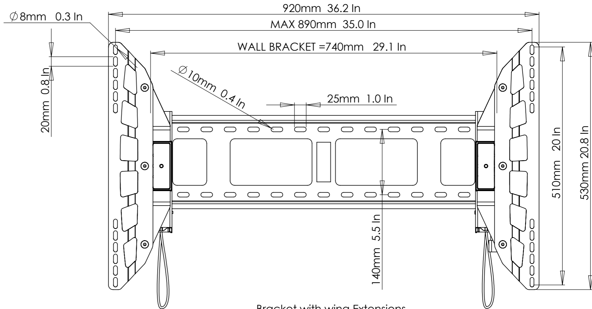
Bracket with wing Extensions
