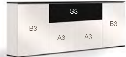
Low Profile 345 88"W x 31.375"H x 12"D Speaker Compartment: 40"W x 11"D x 9"H
